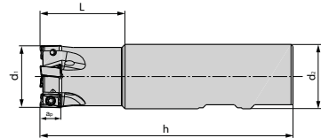
Schaftfräser 90° / LNMX ... End milling cutter 90° / LNMX ...
