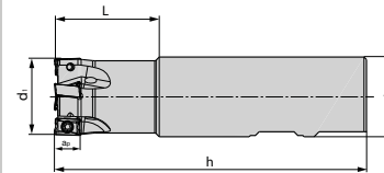
Schaftfräser 90° / LNMX ... End milling cutter 90° / LNMX ....
